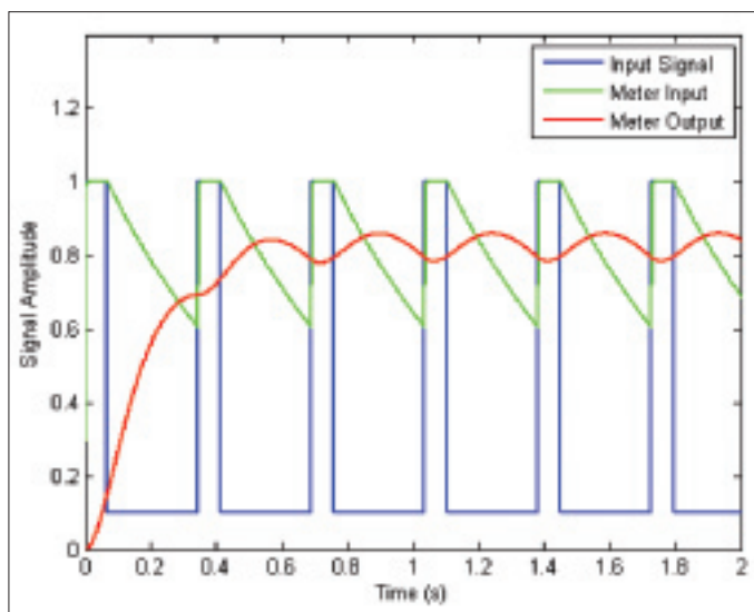
Figure 6. Quasi-peak response to a repetitive signal.
