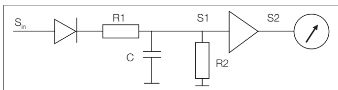
Figure 5. Quasi-peak detector in an analog implementation. The fast-attack (charge time) and slow-decay (discharge time) of the quasi-peak detector result from the R-C constants implemented in this circuit. The resultant waveform drives the critically-damped meter.
