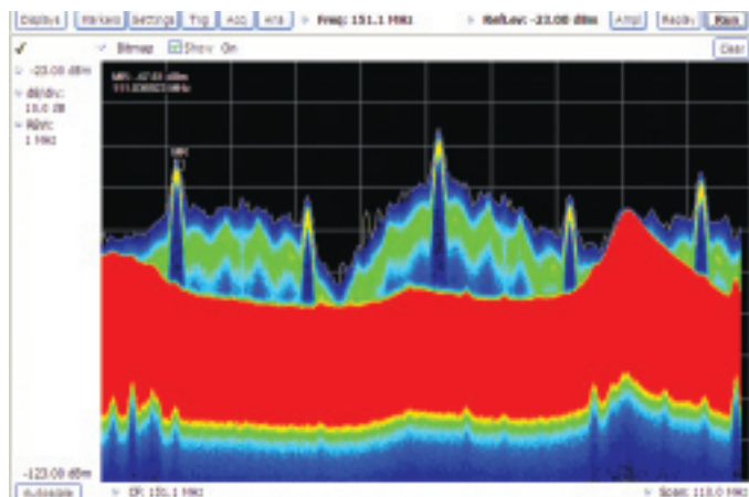
Figure 11. Infrequent transient discovered with DPX after 5 seconds. The red areas are frequently-occurring signals, and the blue and green portions are transients.
