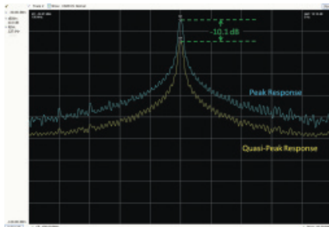
Figure 8. The effect of peak and quasi-peak detection on a signal with an 8 \mu s pulse width and 10 ms repetition rate. The quasi-peak value is 10.1 dB lower than the peak value.
