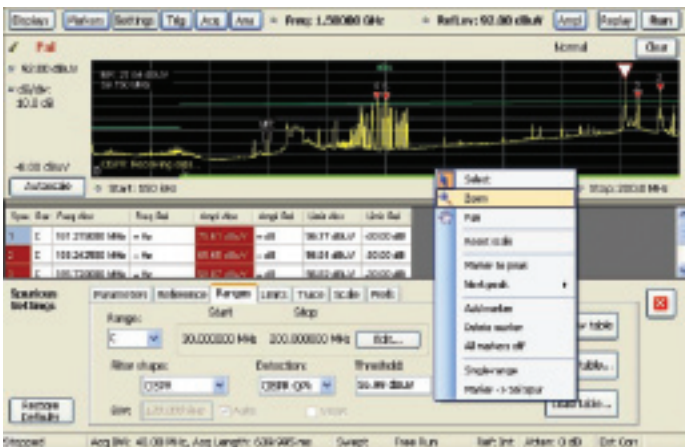
Figure 2. A scan of ambient signals from 150 kHz to 200 MHz. Quasi-Peak detection is used for the entire scan. The spurious measurement in the RSA6100A is set up to change limits vs. frequency, and antenna correction factors have been applied, resulting in the sloped noise floor of the displayed signal. Violations above the user-set limits are shown in red on the table. The menu on-screen can be used to zoom on any portion of the display for closer evaluation.
