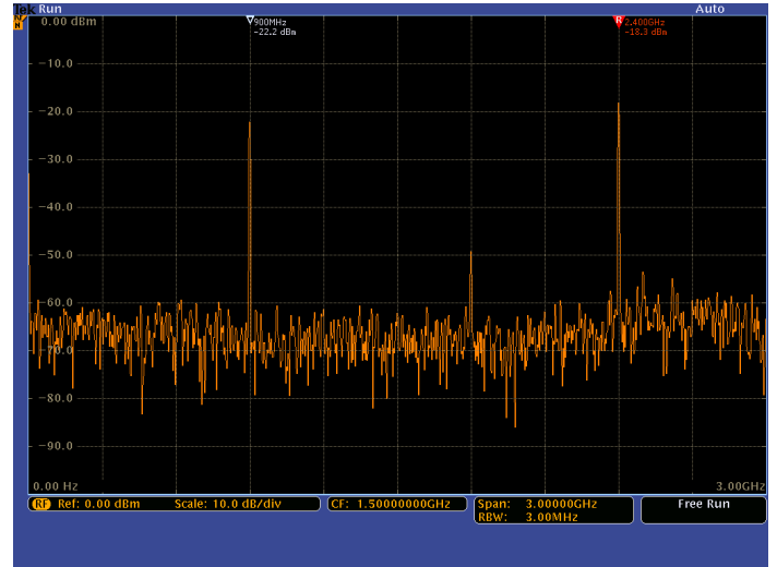
Spectral display of a burst communication both into a device through Zigbee at 900 MHz and out of the device through Bluetooth at 2.4 GHz, captured with a single acquisition.
